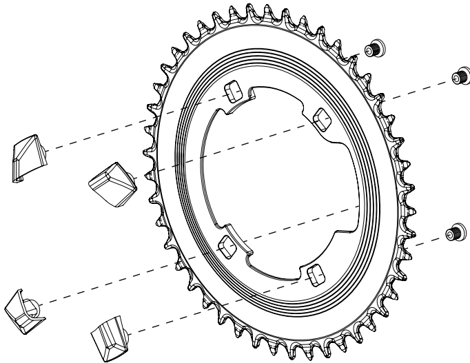
4 Bolt - Semi Speed Ring
